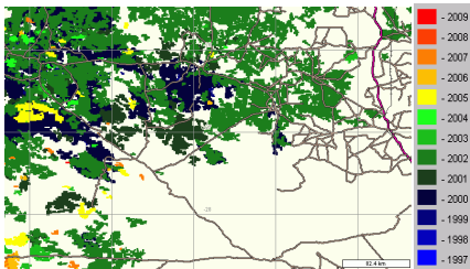
Wildfires in the APY lands between 1997 and 2009.
